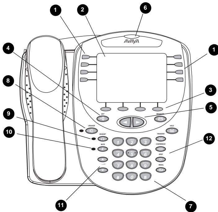
Figure 1: 2420 Telephone Components
